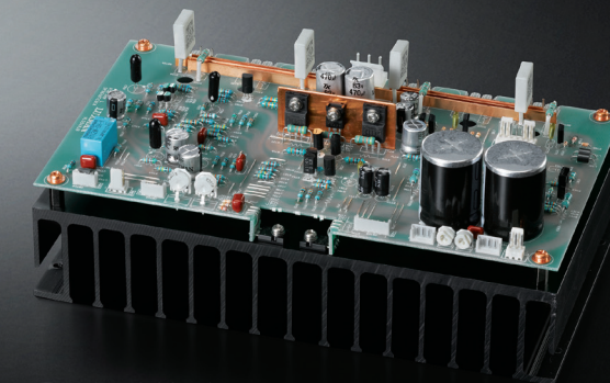
Power Amplifier block of parallel module ODNF version 4.0
