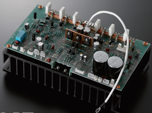
Power amplifier block of 3-parallel module ODNF version 4.0
