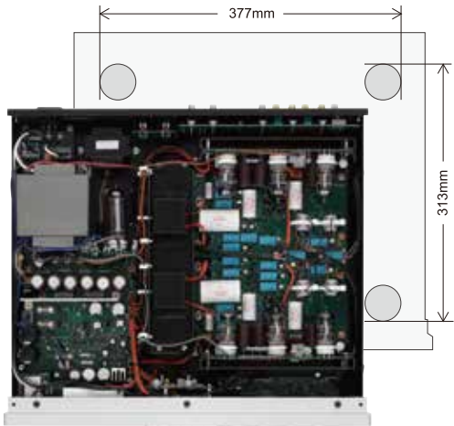
Internal configuration
