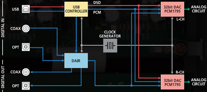
D-05u Conceptual diagram of digital circuit
