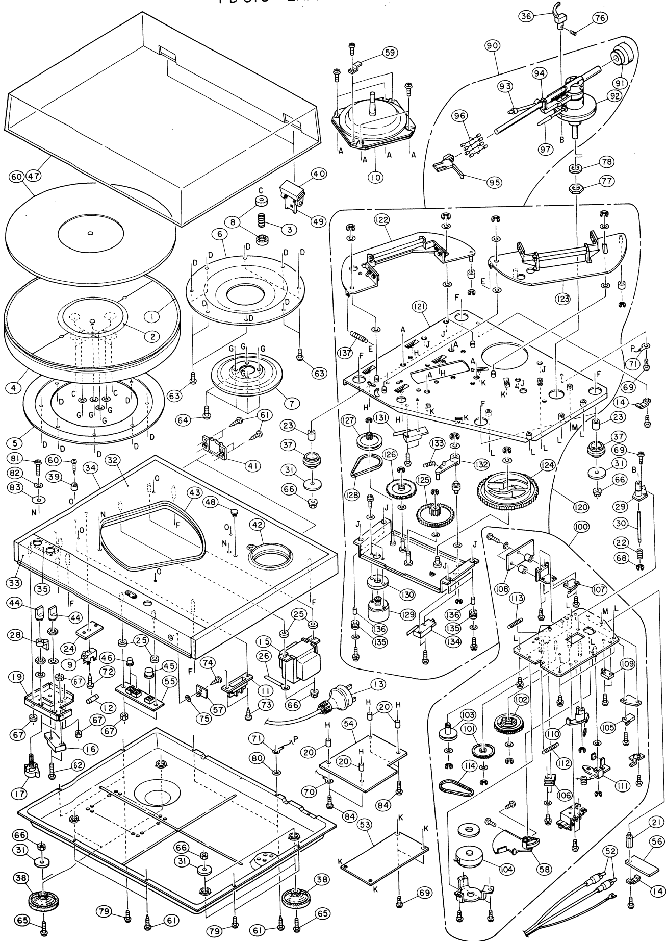
PD-375 EXPLODED VIEW
