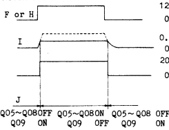
MOTOR SWITCH CIRCUIT TIMING CHART
