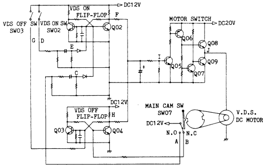
PB-1373 CIRCUIT DIAGRAM
