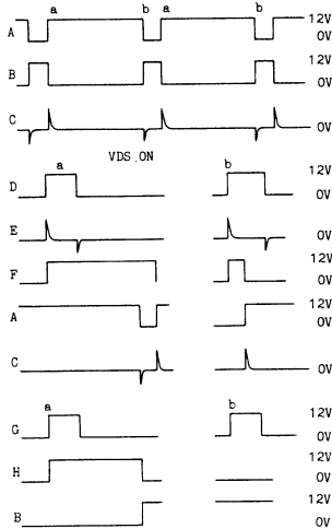
PB-1373 TIMING CHART
