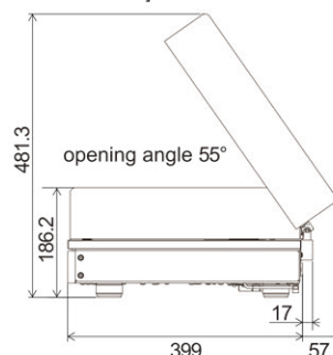
Dimensions with dust cover open [all dimensions are in millimeters]
