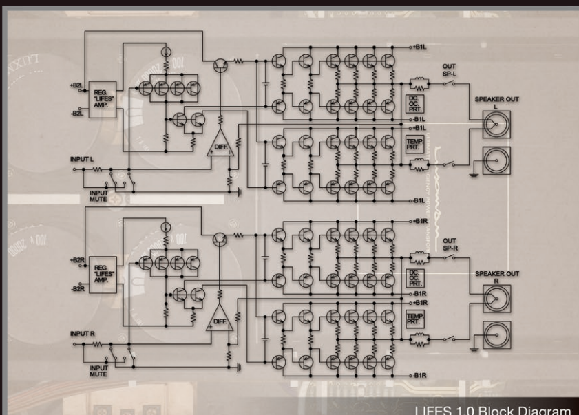
LIFES 1.0 Block Diagram
