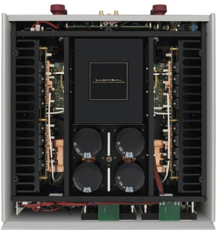
Internal configuration
