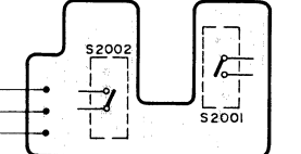
IN/OUT SW P.C. BOARD
