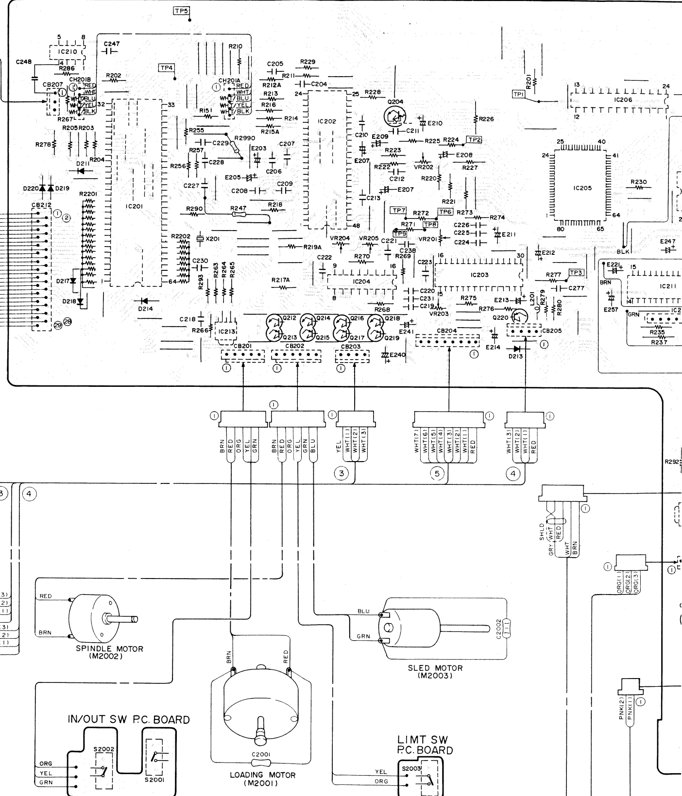
MAIN P.C. BOARD
