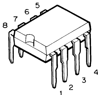
M5216P: IC101
