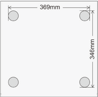
Insulator position / dimensions
