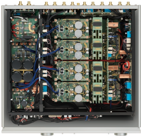
Internal configuration
