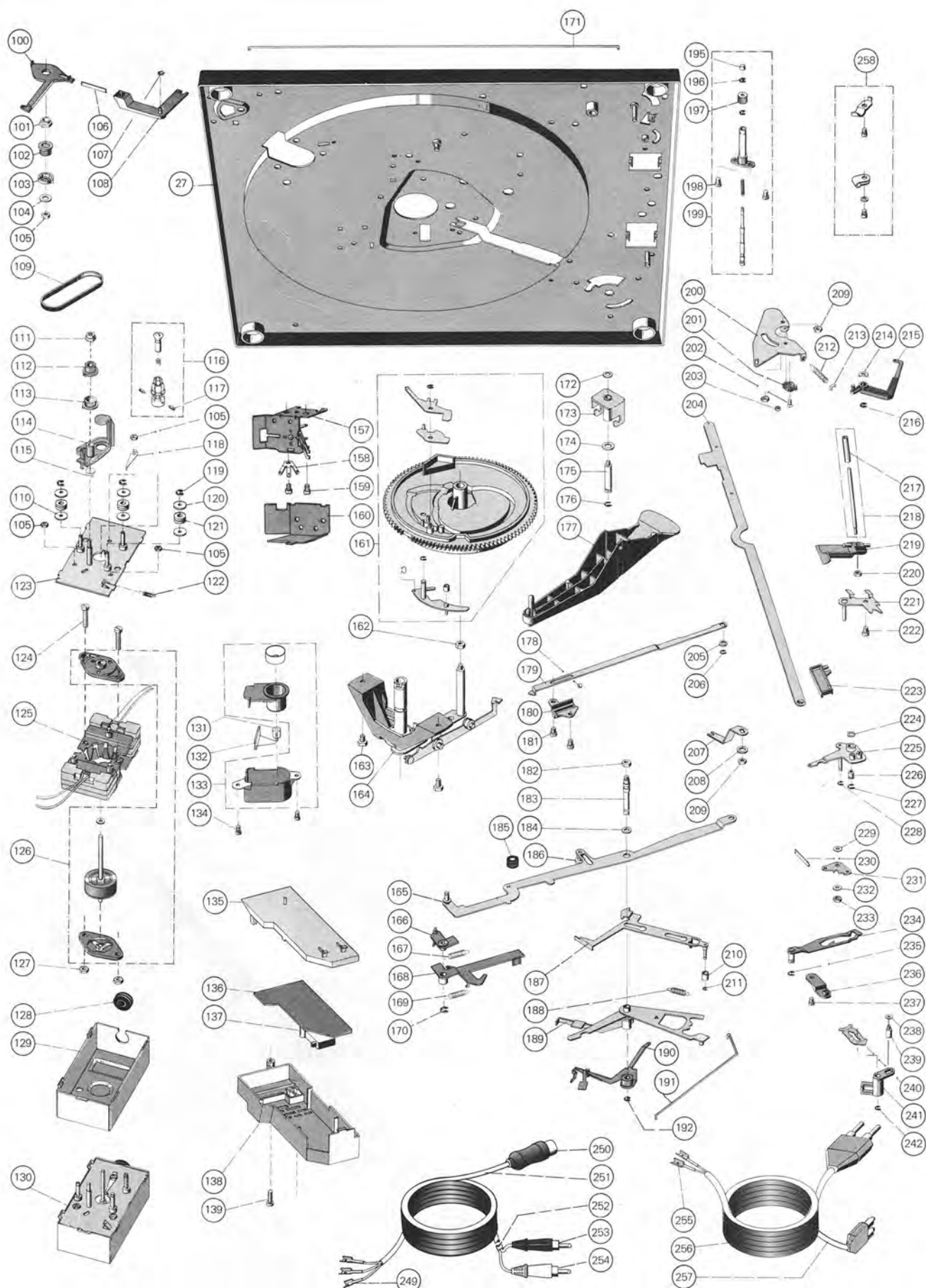
Fig. 21 Exploded view 2
