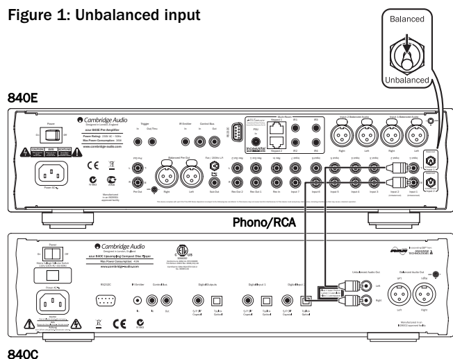
Figure 1: Unbalanced input
