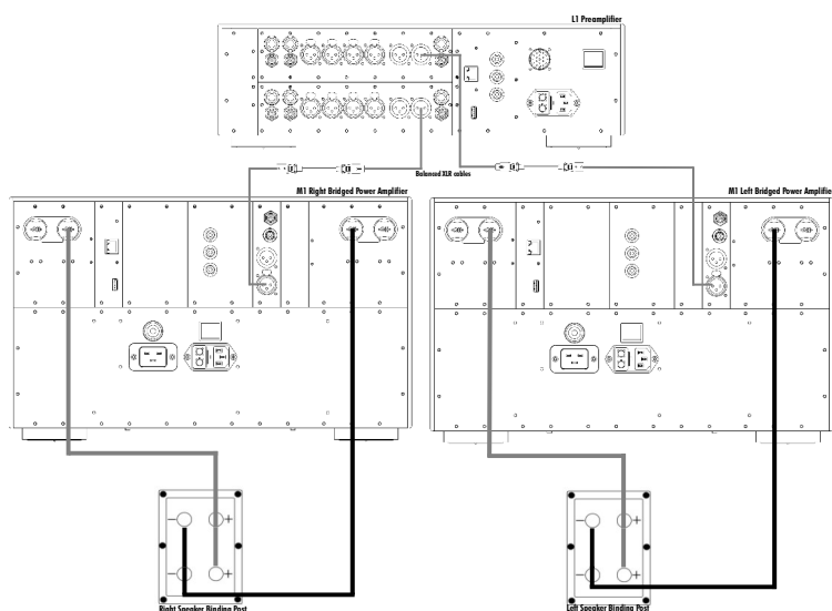
Bridge mode
