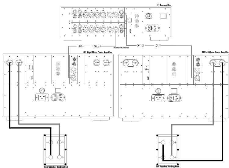
Monaural mode
