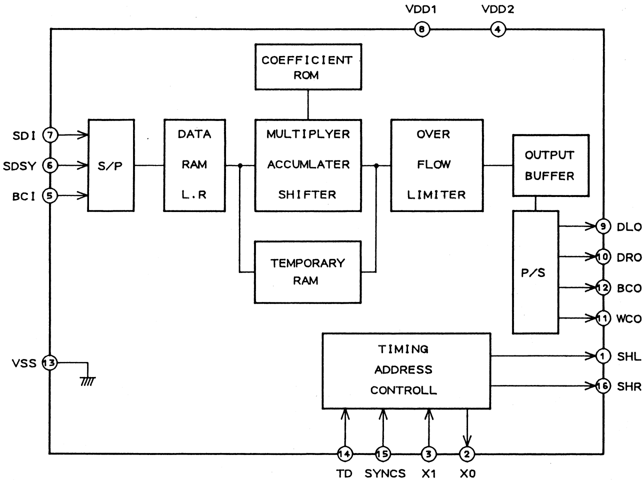
YM3414 (8ft digital firter)
