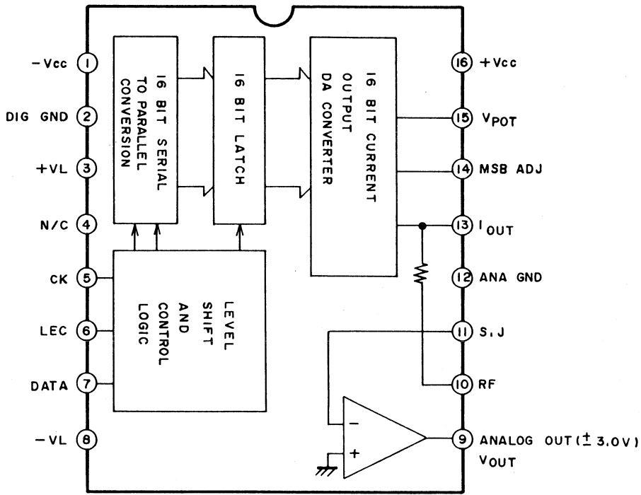
PCM56P (16Bit D/A conveter)
