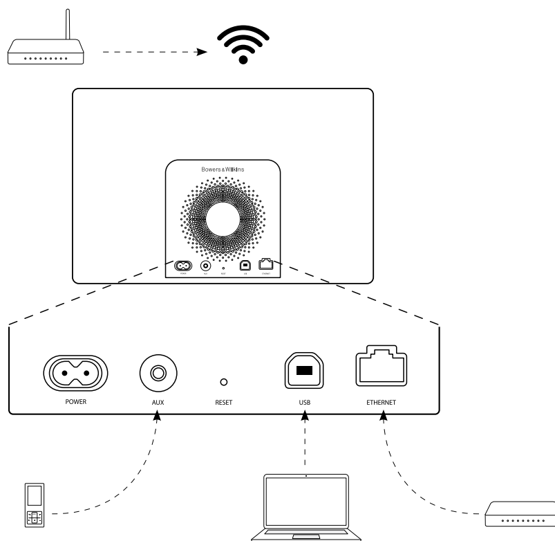
Diagram 5 A7 connectivity
