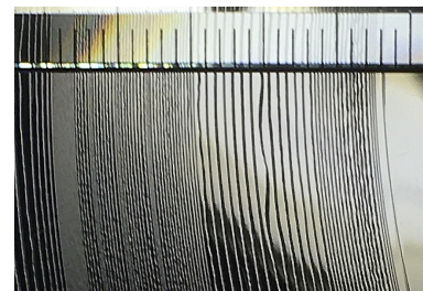
Figure 3.9: An extreme example of a disc in which the groove spacing has been varied to accommodate louder passages in the music. One consequence of this is that this side of the disc contains a single piece of music lasting only 15 minutes and 34 seconds. The ruler at the top of the photo is graduated in mm.
