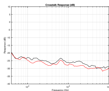
Figure 5.4: Results from a crosstalk measurement. The result of this measurement was -25.3 dB.
