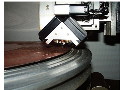
Figure 3.11: A Neumann-Teldec cutting head creating the groove in the master disc. The cutting stylus shown in Figure 3.10 can be seen just under the circular support under the head. (Wikimedia Commons)
