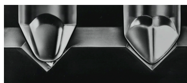
Figure 3.18: An example of an elliptical stylus on the left vs. a line contact Pramanik grind on the right. Notice the difference in the area of contact between the styli and the groove walls.
