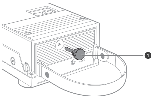
① Tonearm fixing screw
