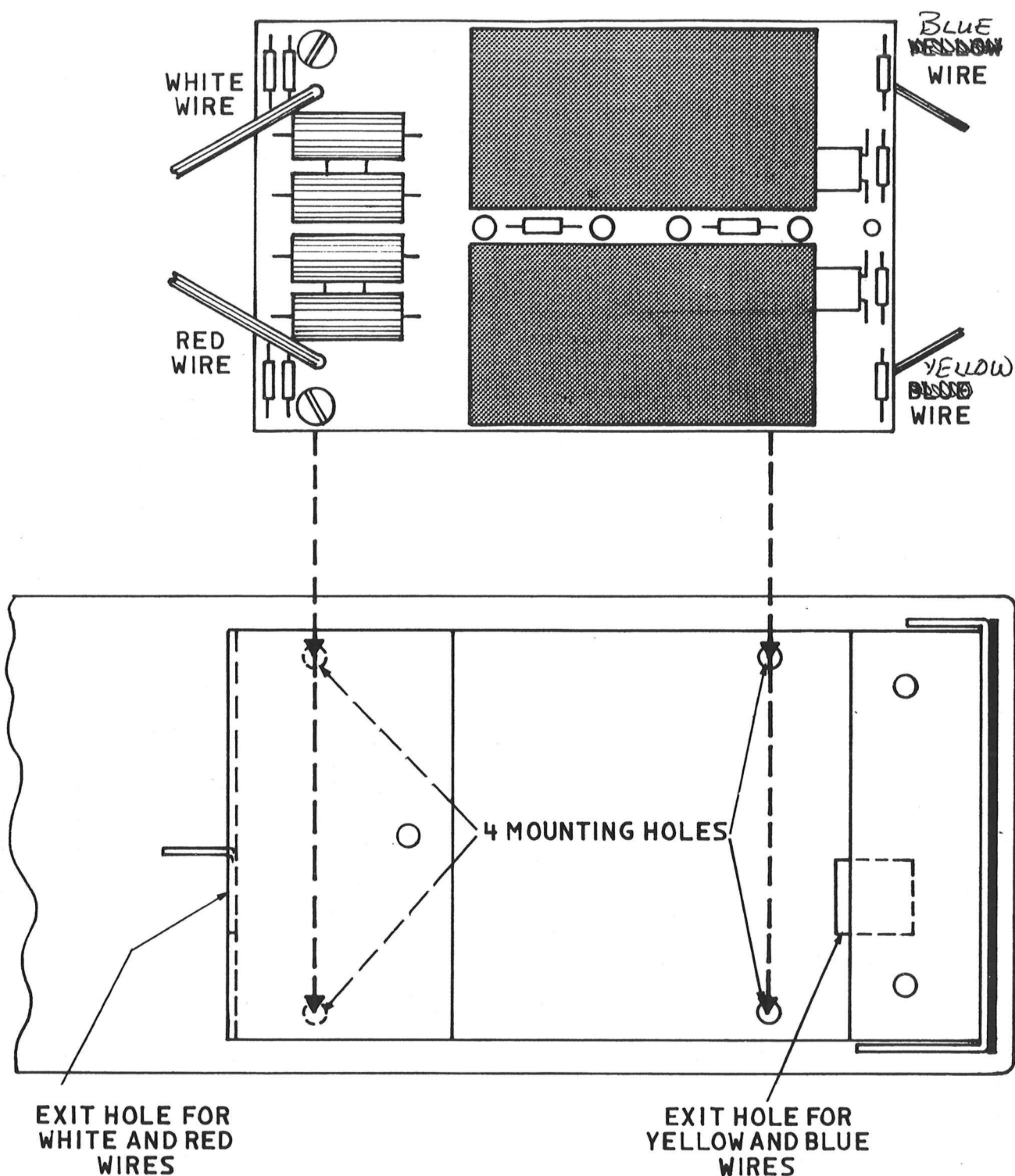
PREAMPLIFIER END VIEW (SIDE PANELS REMOVED)
