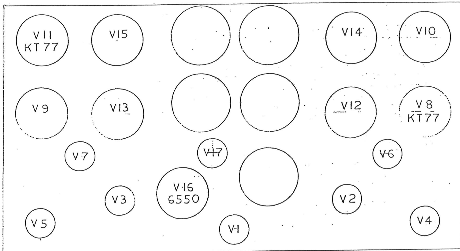
VACUUM TUBE LOCATIONS D115 AMPLIFIER
