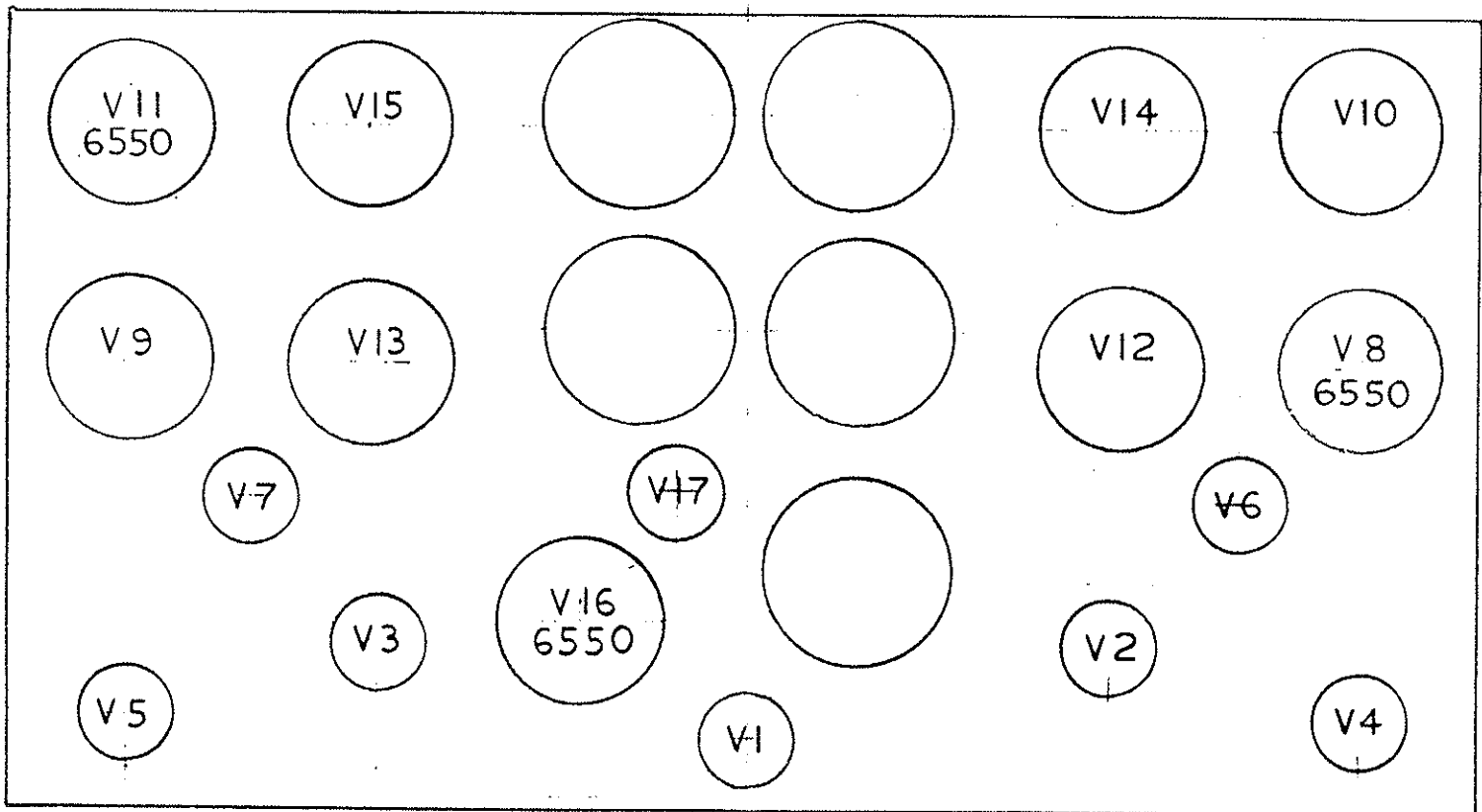
VACUUM TUBE LOCATIONS D115MKII AMPLIFIER
