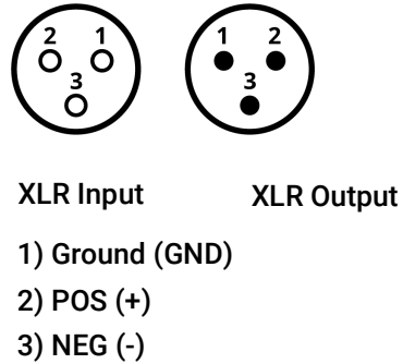
Abb. 3. Assignment of XLR connectors
